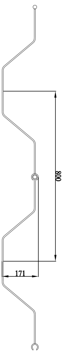
INTERLOCKED PROFILE
