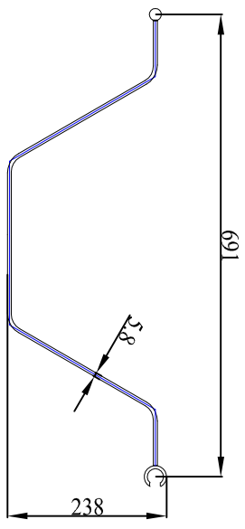
SHEET PILE PROFILE
