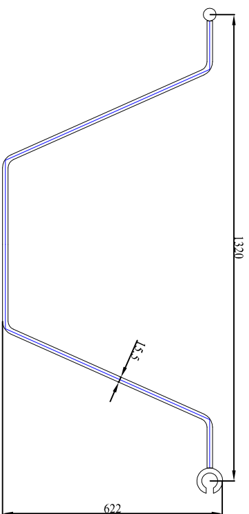
SHEET PILE PROFILE
