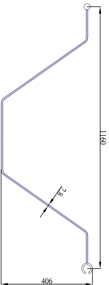
SHEET PILE PROFILE
